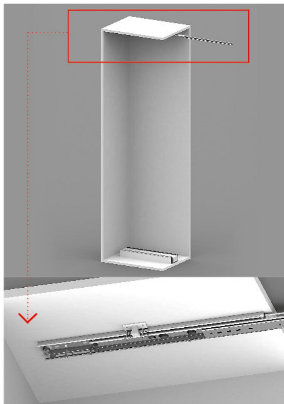
Step 02 : Fix Top Slider and Soft-Close Lock with carcass using Top Template and Fitting Kit - 1.
