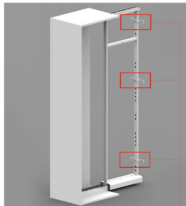
Step 12 : With the help of Bracket Cover, lock all the Baskets.
