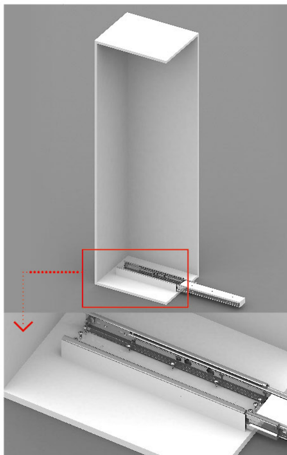
Step 01 : Fix Bottom Slider with carcass using Bottom Template and Fitting Kit - 1.
